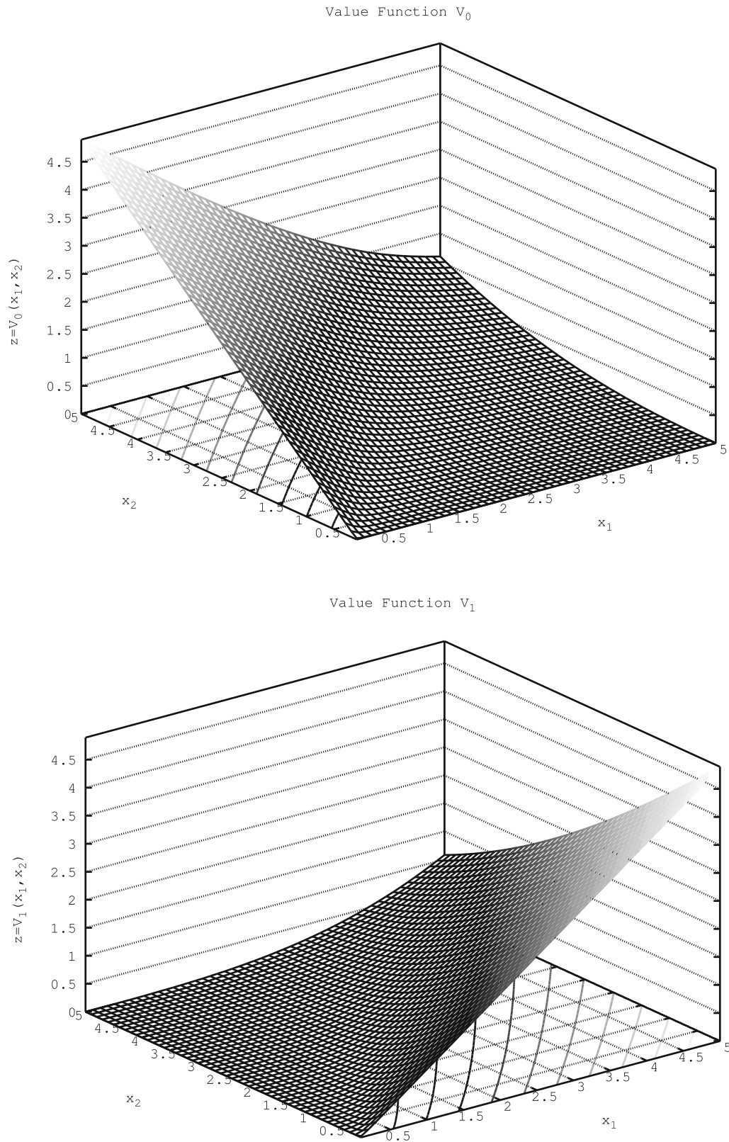
Fig. 3 Value functions
